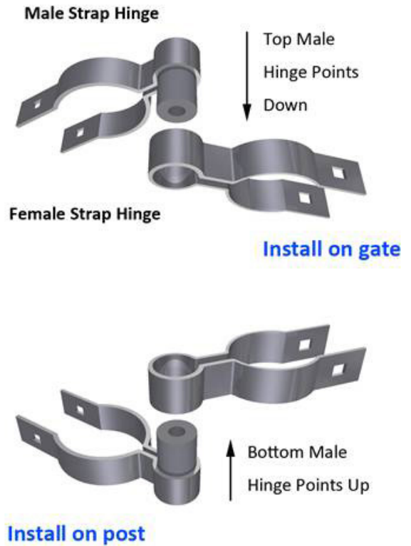
Installation picture of gate frame hinges
