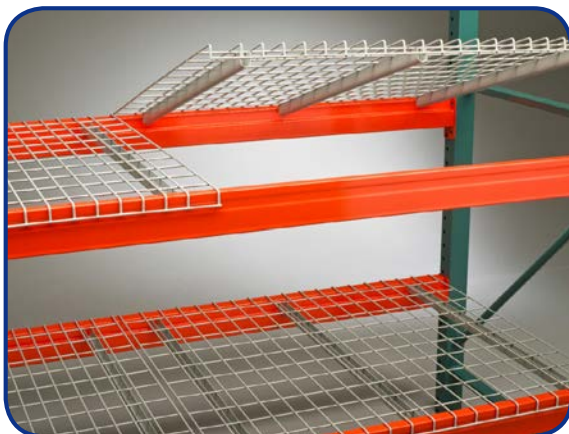
Wire decking installed on support frame
